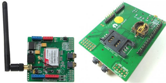
Figure 3. Shield GSM/GPRS SIM900 / Placa GSM/GPRS SIM900
