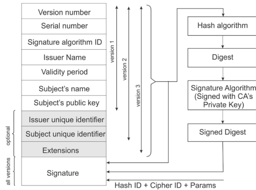
Figure 3. X.509 Certificate Format / Formato certificado X.509
