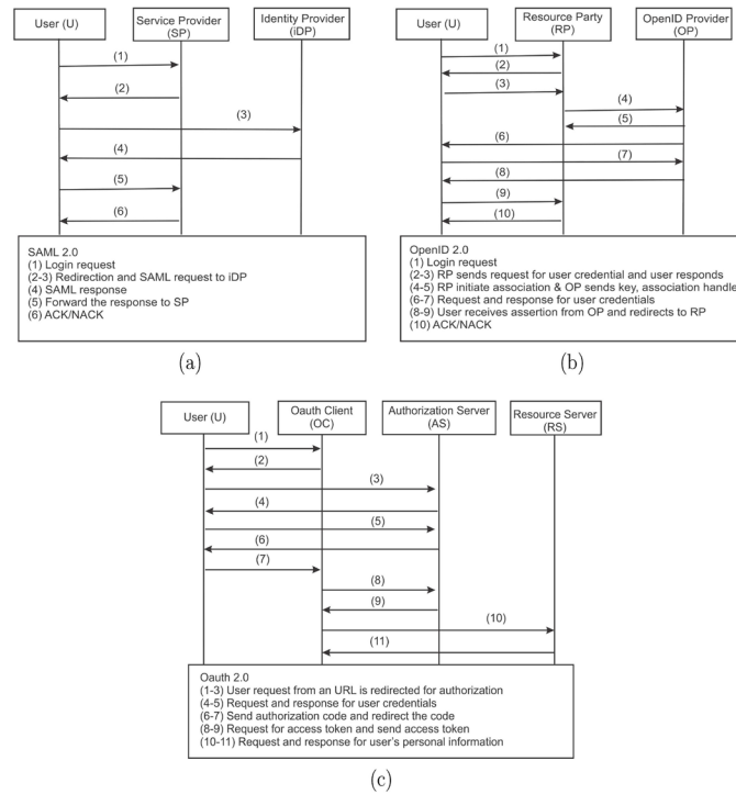
Figure 2. Token based authentication using SAML (a), OpenID 2.0 (b) and OAuth 2.0 (c) Autenticación basada en tokens usando SAML (a), OpenID 2.0 (b) y OAuth 2.0 (c)
