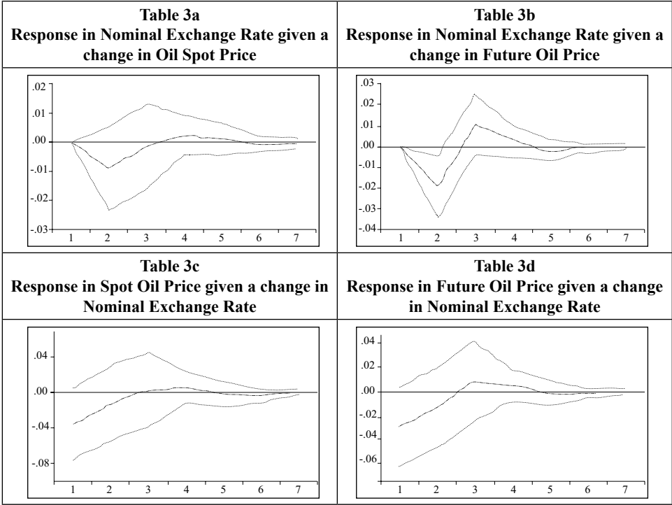
Figure 3 Impulse-Response Functions
