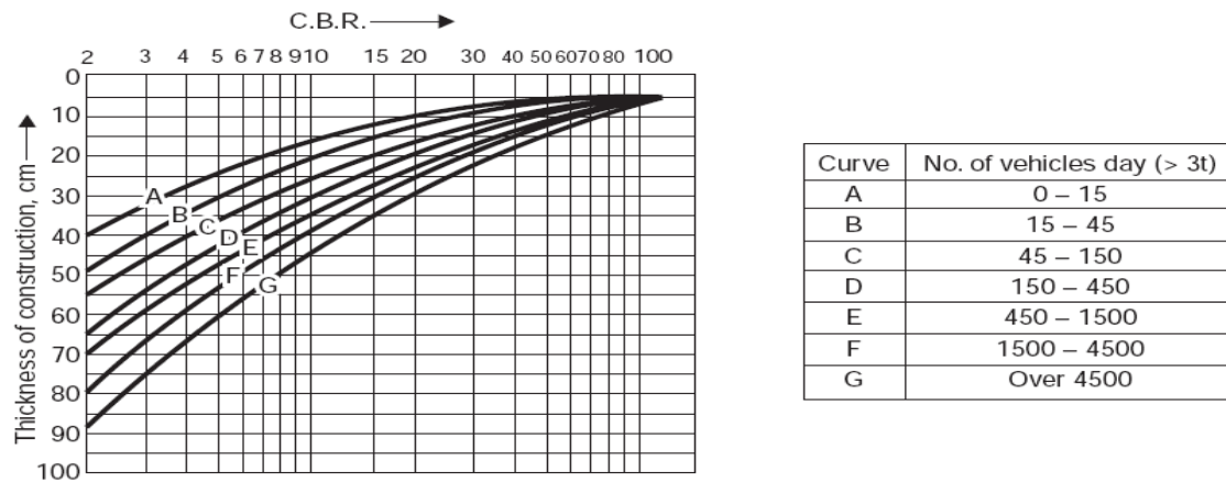
Fig. 17.4 Design charts for flexible pavements—CBR method (After R.R.L., London & Alam Singh, 1967)
