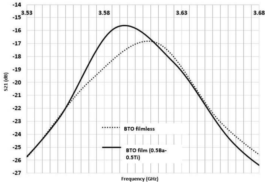
Fig. 8 Close up to the first peak of fundamental resonance of the CPW resonator with and without BTO content.
