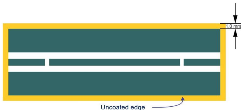
Fig. 3 Isolated borders of the CPW resonator.
