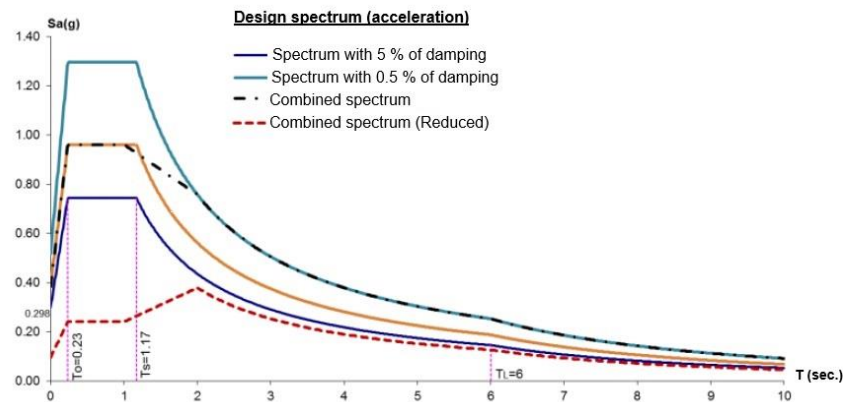
Fig. 1. Acceleration Spectrum.
