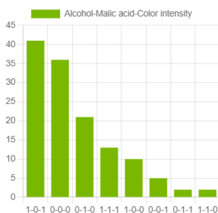
Fig. 6. Combinatorial count result "Alcohol, Malic acid, Color intensity".
