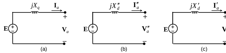
Fig. 5. Model of constant voltage behind reactance of the SM. (a) Steady state, (b) Sub transient state, and (c) Transient state.
