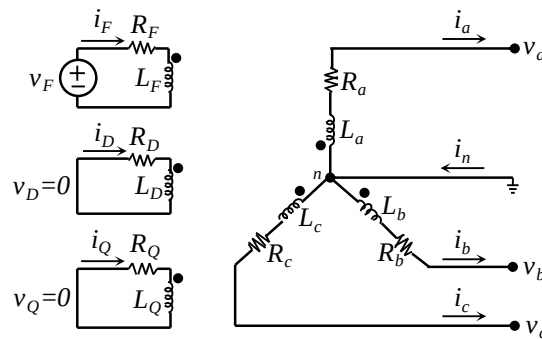
Fig. 2. Mutually coupled circuits of a SM in the abc domain.
