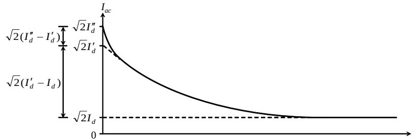
Fig. 4. Envelope of the armature current I_{ac} for the SSC fault [15].
