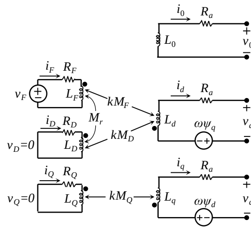
Fig. 3. Mutually coupled circuits of the SM in the dq domain [15].
