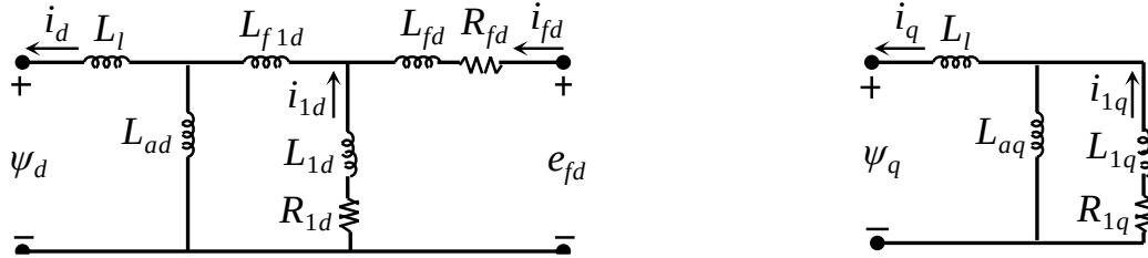
Fig. 6. Equivalent circuits referred to the stator for the 2.1 model of the SM [21].
