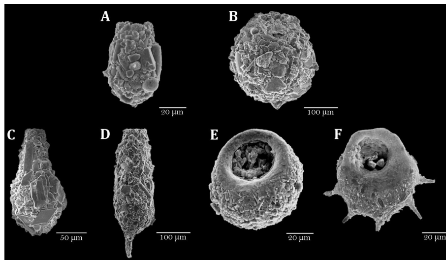
Figure 3. Scanning electron microscopy images of selected species of testate amoebae in the sediments from lakes El Sol and La Luna, Nevado de Toluca, central Mexico. A, Diffugia glans strain “glans”; B, Diffugia globulosa ; C, Diffugia oblonga strain “oblonga”; D, Diffugia protaeiformis strain “acuminata”; E, Centropyxis constricta strain “aerophila”; F, Centropyxis constricta strain “spinosa”.
