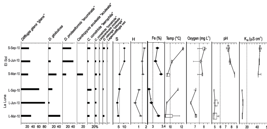
Figure 2. Main testate amoebae taxa (> 3%), species richness (S), Shannon diversity (H) and Fe concentrations in surface sediment samples from lakes El Sol (top) and La Luna (bottom), Nevado de Toluca, central Mexico. The graph also shows boxplots of water column parameters: temperature (Temp.), oxygen concentrations, pH and electric conductivity ( K_{25} ).
