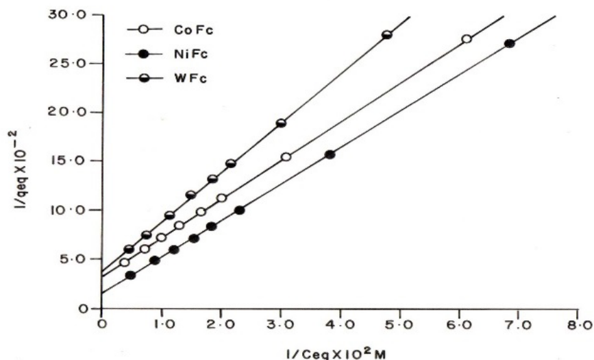
Fig. 7. Langmuir plots of 2-nitrophenol on metal ferrocyanides. Temperature = 30 \pm 1^\circ\text{C} ; pH = 7.0 \pm 0.01 ; amount of metal ferrocyanide = 25 mg; particle size = 125 \mu\text{m} ; \lambda_{\text{max}} 2-nitrophenol = 360 nm; CoFc = cobalt ferrocyanide; NiFc = nickel ferrocyanide; WFc = tungsten ferrocyanide.
