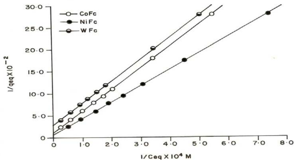
Fig. 8. Langmuir plots of 2,4-dinitrophenol on metal ferrocyanides. Temperature = 30 \pm 1^\circ\text{C} ; pH = 7.0 \pm 0.01 ; amount of metal ferrocyanide = 25 mg; particle size = 125 \mu\text{m} ; \lambda_{\text{max}} 2, 4-dinitrophenol = 360 nm; CoFc = cobalt ferrocyanide; NiFc = nickel ferrocyanide; WFc = tungsten ferrocyanide.
