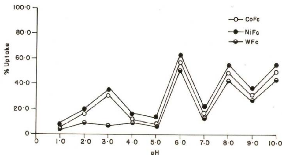
Fig. 1. Effect of pH on adsorption of 2-nitrophenol on metal ferrocyanides. Temperature = 30 \pm 1^\circ \text{C} ; pH = 1.0\text{--}10.0 \pm 0.01 ; amount of metal ferrocyanide = 25 mg; particle size = 125 \mu\text{m} ; \lambda_{\text{max}} 2-nitrophenol = 360 nm; CoFc = cobalt ferrocyanide ; NiFc = nickel ferrocyanide ; WFc = tungsten ferrocyanide .
