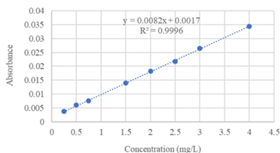
Figure 2. Analytical calibration curve for the lead (Pb) in HNO 3 1 % (v/v).
