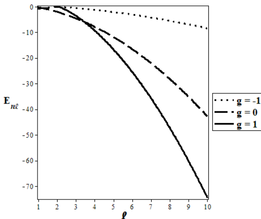
Figure 8. Energy Eigenvalue Variation with \ell for different values of g with D = 3, \alpha = 1, A = 5, n = 0 .
