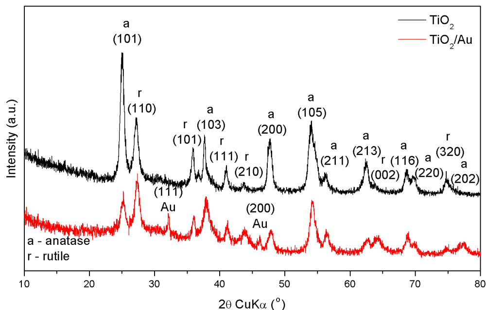
Figure 4. \text{TiO}_2/\text{Au} nanoparticles XRD patterns.
