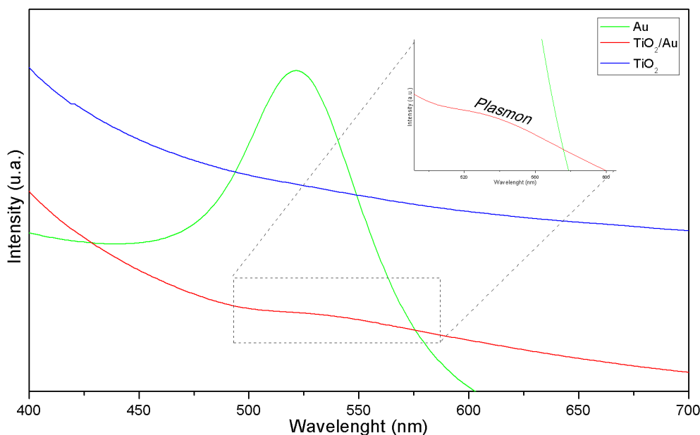
Figure 5. \text{TiO}_2/\text{Au} , \text{TiO}_2 and Au nanoparticles UV-Vis spectra.
