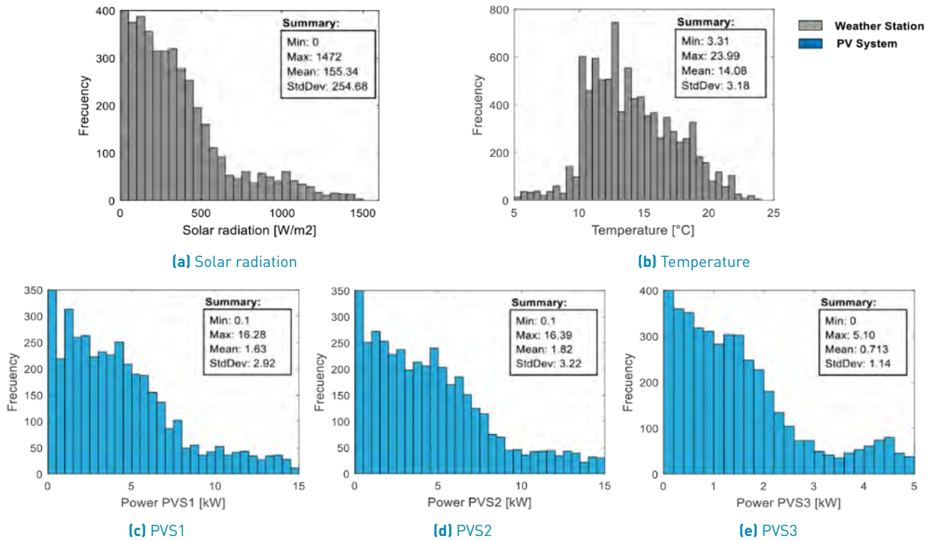
Figure 7 Histograms of the meteorological variables
