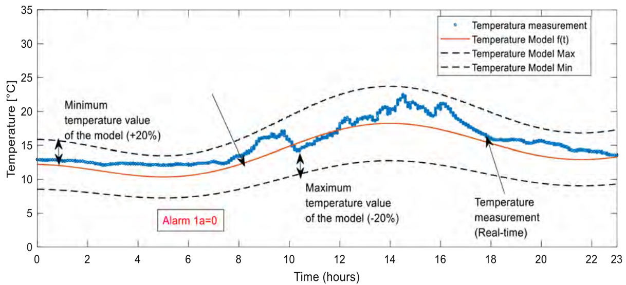
Figure 16 Monitoring algorithm for temperature measurement
