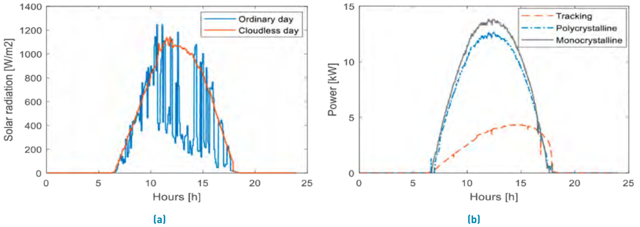
Figure 9 (a) Impact of cloudiness on radiation, (b) Photovoltaic power PVS1, PVS2 and PVS3 (clear day)
