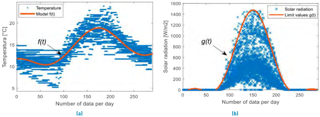
Figure 8 (a) Temperature and (b) Solar radiation, during one-month weather station (Test phase -August 2018)
