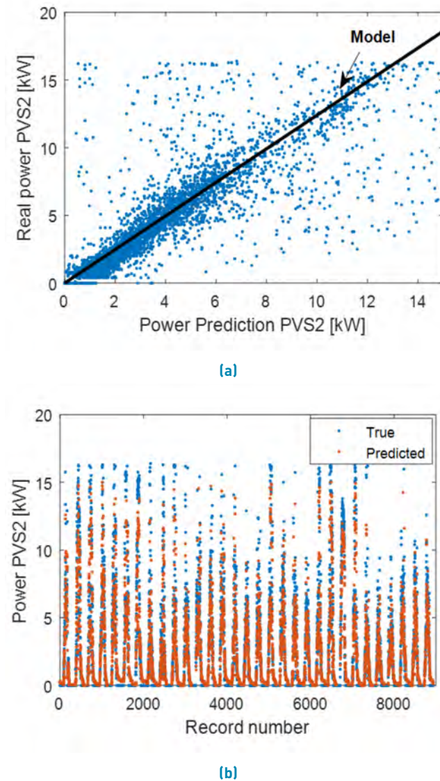
Figure 13 (a) Regression model applied to PVS2, (b) Phase validation PVS2
