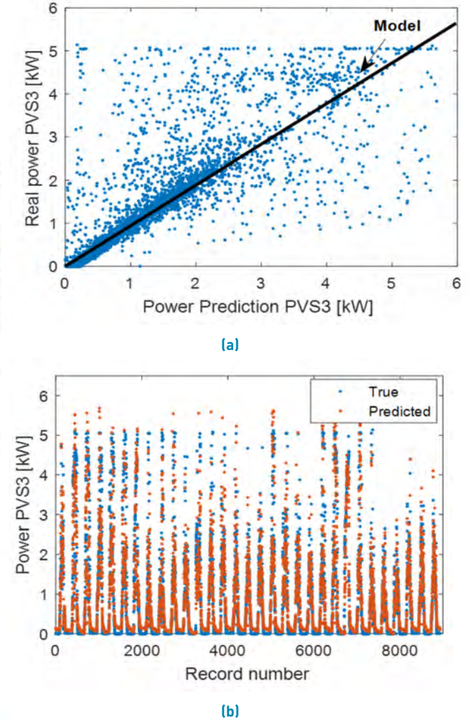
Figure 14 (a) Regression model applied to PVS3, (b) Phase validation PVS3
