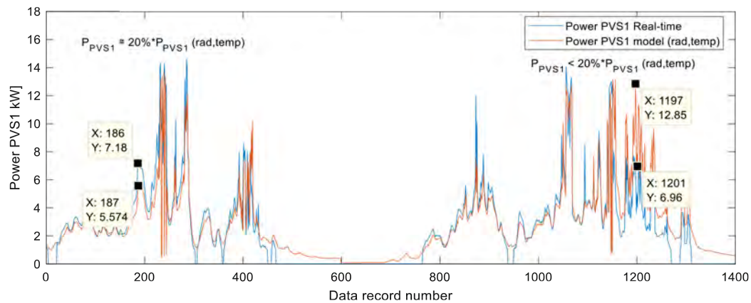
Figure 19 Algorithm application for PVS1 system (two days of registration)
