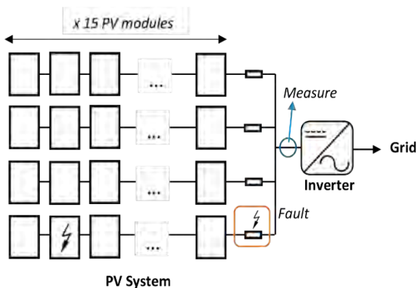
Figure 18 Fault simulation in a branch of the PVS1 system
