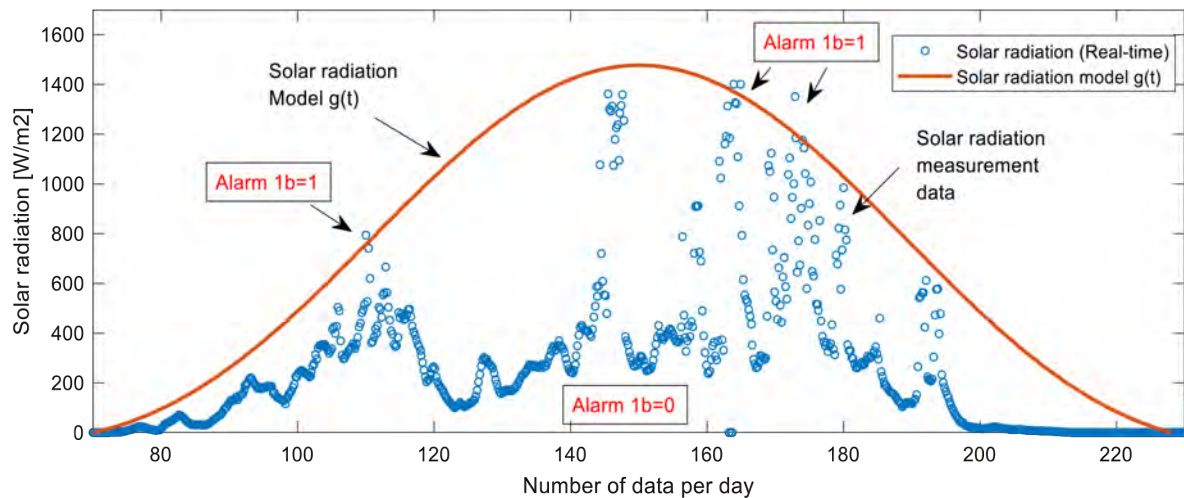
Figure 17 Monitoring algorithm for measuring solar radiation
