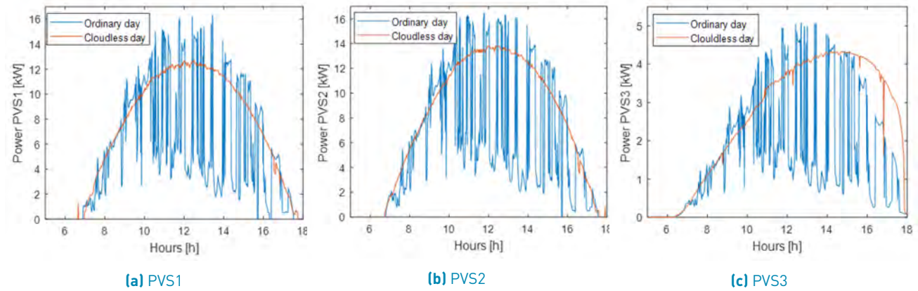
Figure 10 Comparison in the PV generation against an ordinary and clear day
