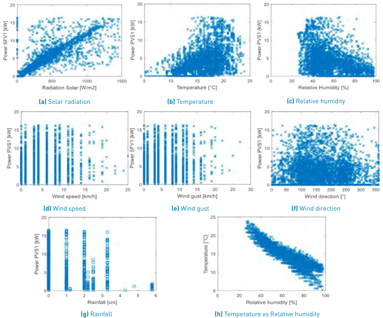
Figure 6 Power PVS1 according to the variables of the weather station
