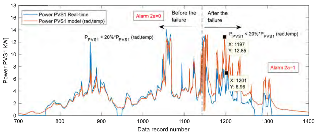
Figure 20 Algorithm application before and after a failure (12 hours of registration)
