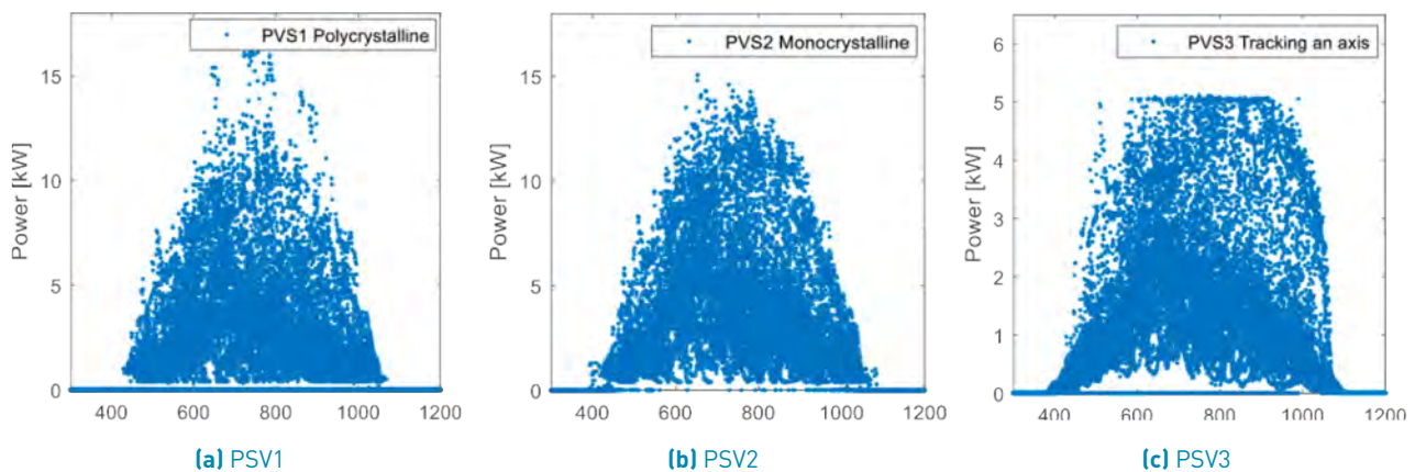
Figure 5 Power generated during one month (July 2018)
