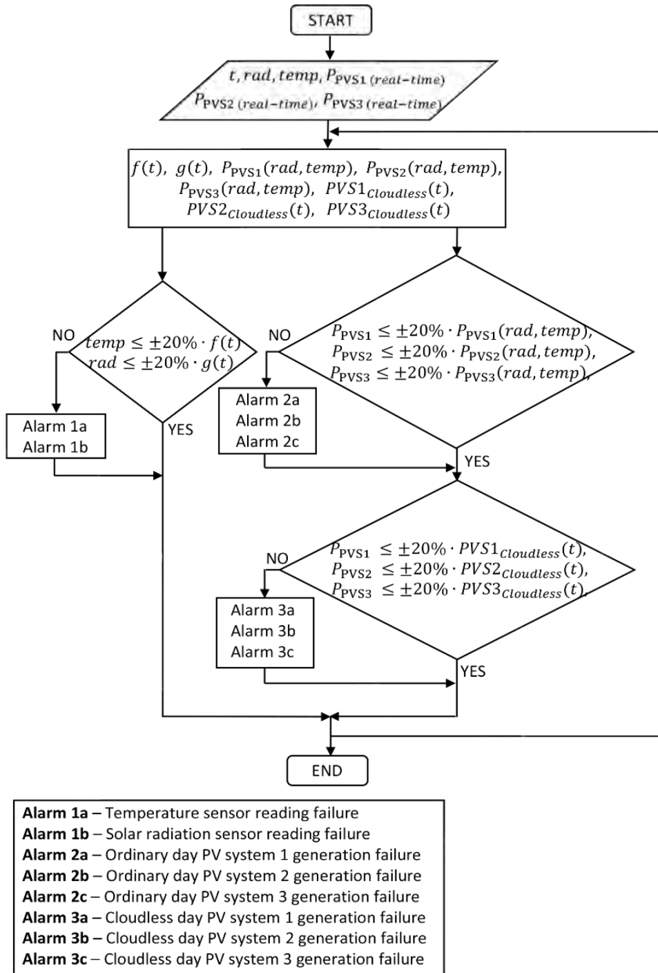
Figure 15 Algorithm for monitoring and fault detection with alarm indicators
