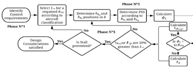
Figure 7 Ailerons design methodology workflow diagram
