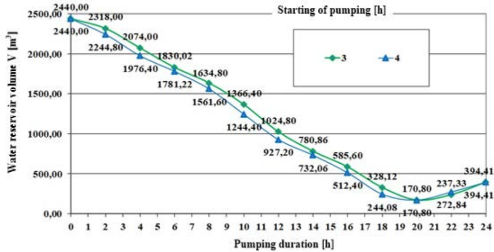
Figure 6 Dependence of the required water tank volume on the pumping duration for different pumping start for Q_{max}^{daily} = 2440 m^3/day for extremes (minimum values of water tank volume) with pumping starts at 3 and 4 AM for Variant I
