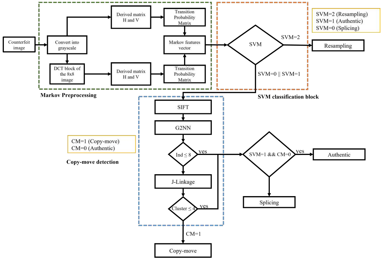
Figure 1 General flow diagram of the proposed algorithm
