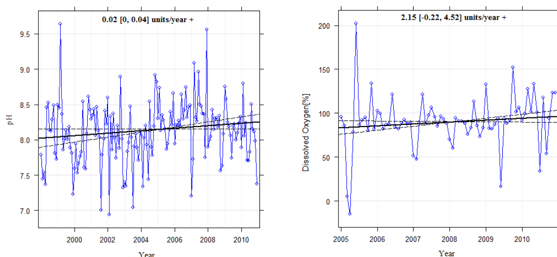
Figure 5 Confidence intervals and the threshold of significance of the Theil-Sen slope of trends in pH and DO
