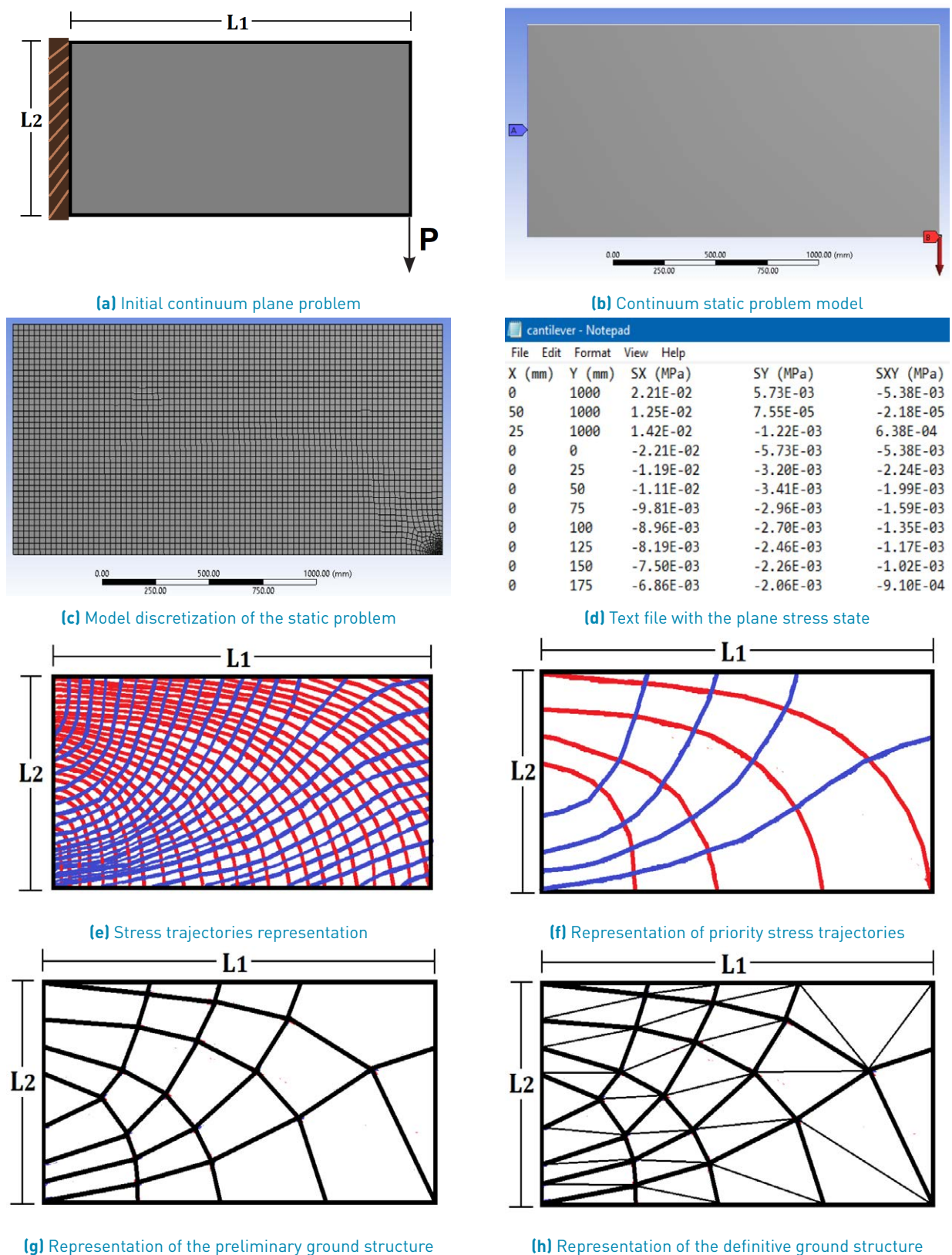
Figure 2 Steps to generate the ground structure
