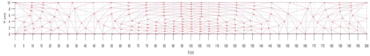
Figure 11 Definitive ground structure for the 200 m span continuous bridge
