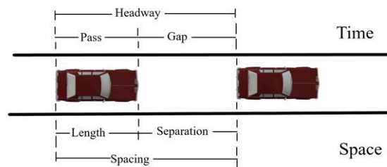
Figure 1 Microscopic variables
