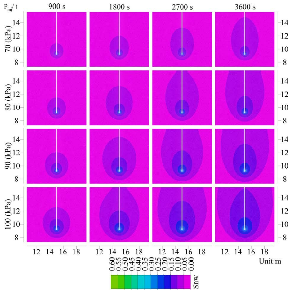
Figure 4 Isocountours-distribution of S_{nw} due to changes in P_{nw,inj} . Distance in meters
