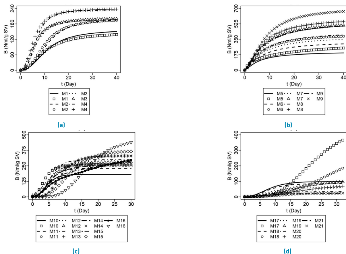
Figure 2 ACoD kinetics of experimental substrates (markers) and kinetics defined by the additive model (lines). (A) [10], (B) [12], (C) [22], (D) [23]
