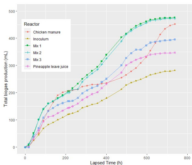
Fig. 2. Total biogas production during the biomethane potential test.
