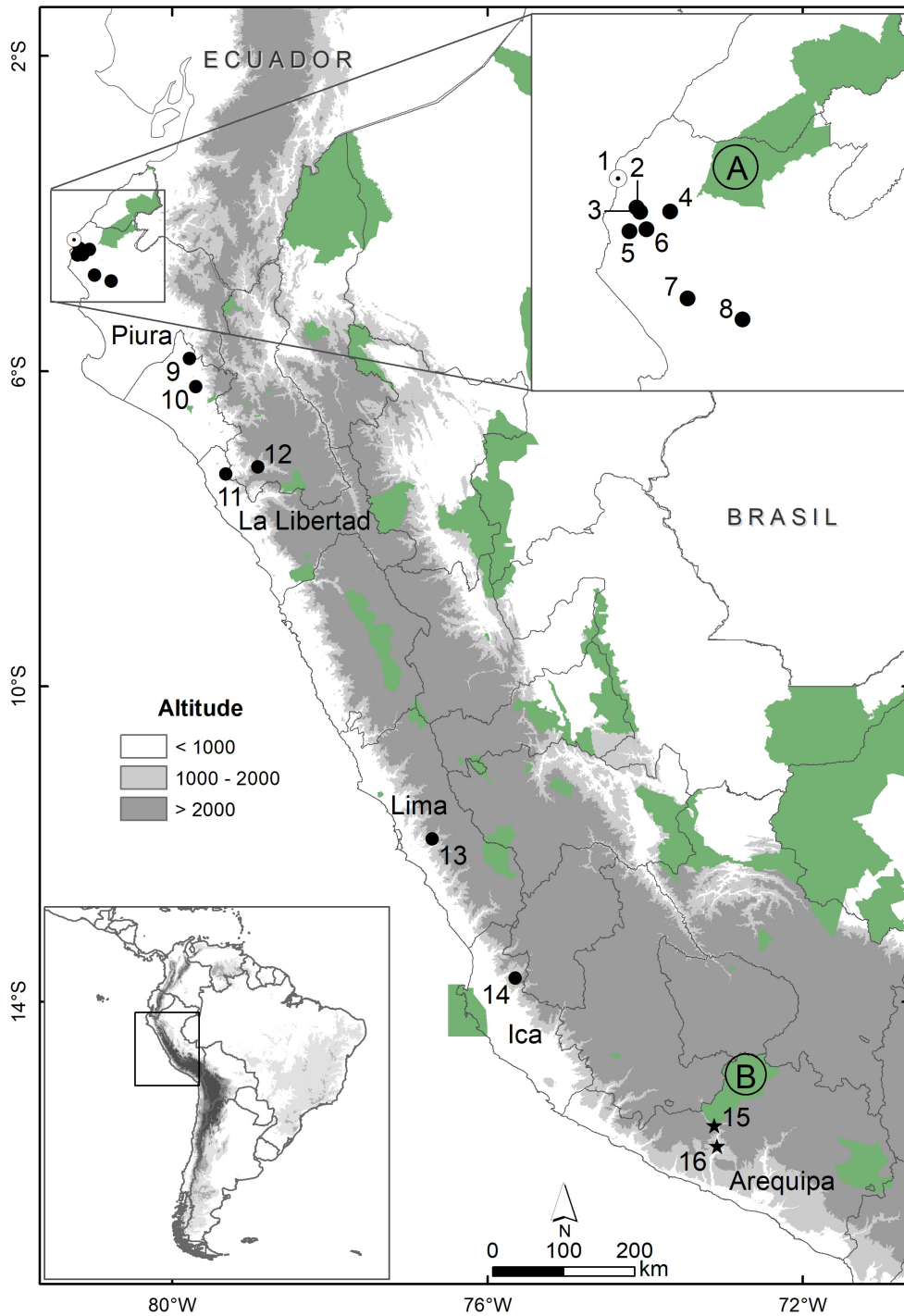
Fig. 1. Map showing known localities of Tomopeas ravus . Previous records (black dots) (Velazco et al. 2013); new records in the north, Alto Talara, Piura (white dot); and in the south, Ocoña Valley, Arequipa (stars). The Peruvian protected natural areas pointed out in green. Protected natural areas nearest to T. ravus records: A. Coto de Caza El Angolo; B. Reserva Paisajística Sub Cuenca del Cotahuasi. The name of localities is given in the Appendix 1 .
