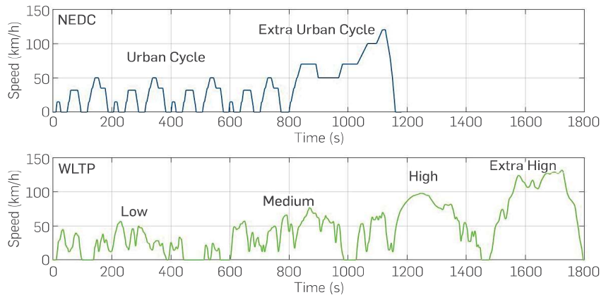
Figure 2. Speed profiles of NEDC and WLTP [5]
