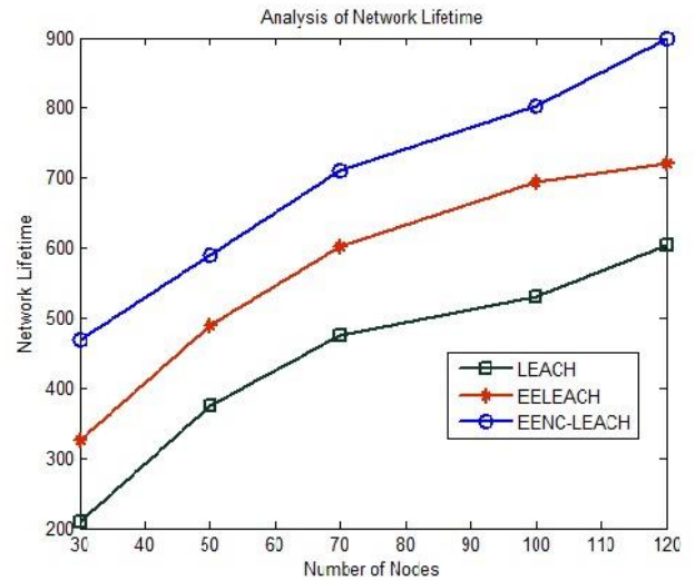
Fig. 3. Network Lifetime with respect to number of nodes.
