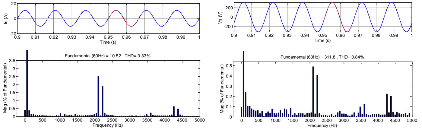
Fig. 10. 36-pulse AC-DC converter input current and voltage waveforms at light load condition including the harmonic spectrum.
