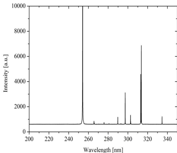
Fig. 3. Characterization of the ultraviolet radiation lamp.
