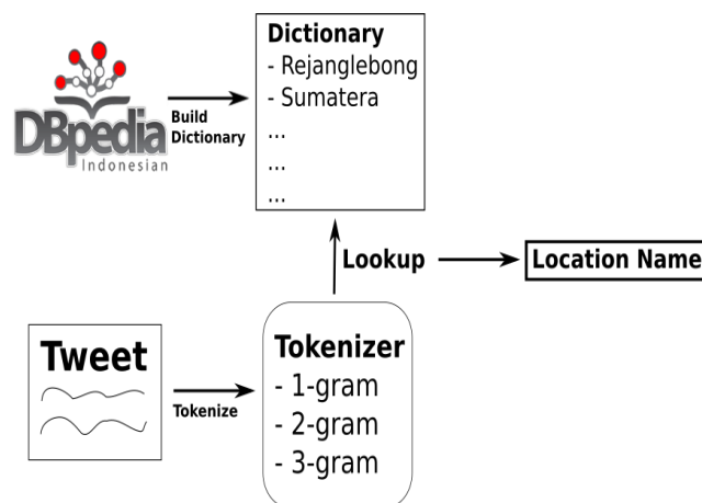
Figure 2. Location entity recognizer.
