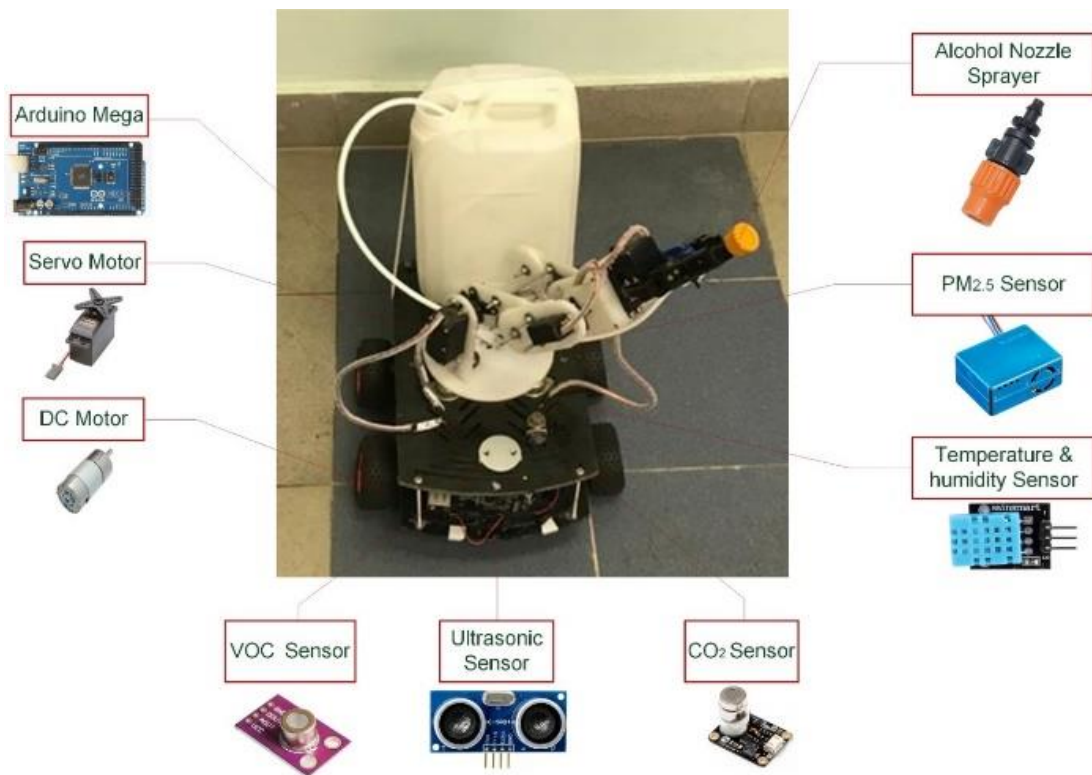
Figure 3. Experimental system setup.
