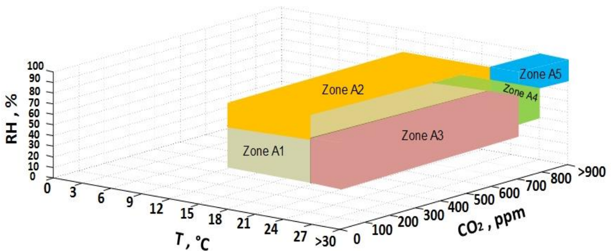
Figure 6. "A" zones for (T, RH & CO 2 ).
