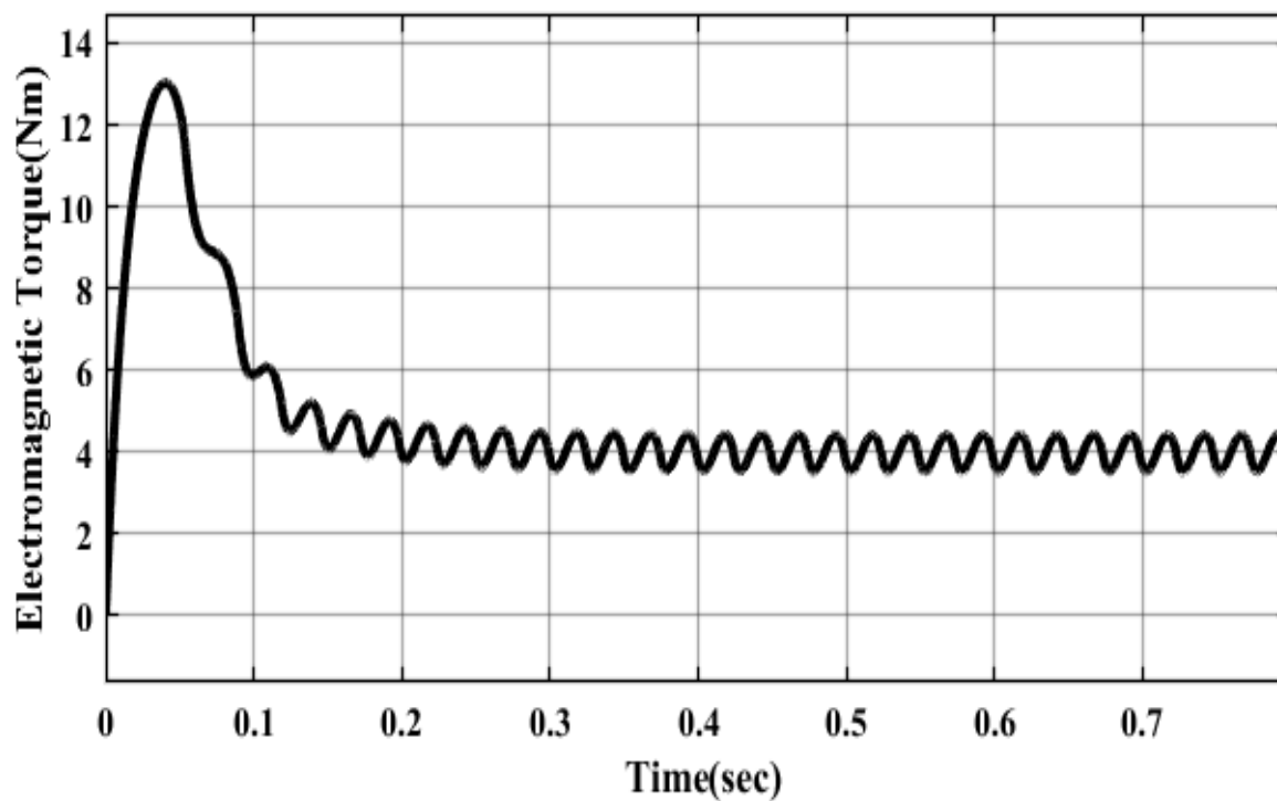
Figure 12. Torque responses vs. time for the detailed closed-loop model utilizing the classical controllers.
