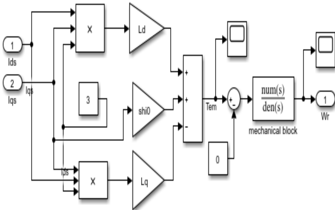
Figure 11. MATLAB simulation arrangement of the mechanical subsystem block.
