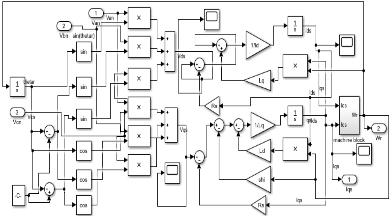
Figure 10. MATLAB simulation arrangement of the machine block subsystem block.
