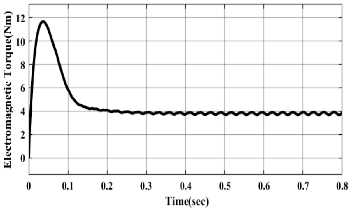
Figure 21. Electromagnetic torque Vs. Time for detailed closed-loop model utilizing particle swarm optimization.
