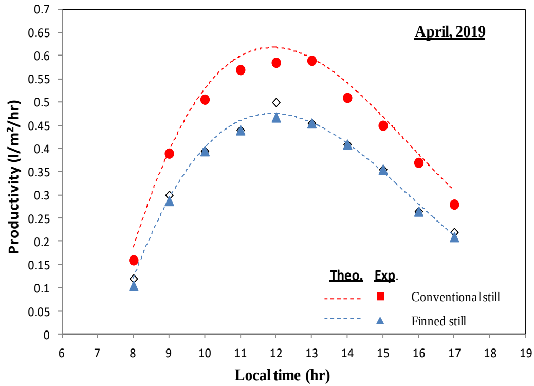
Figure 13. Hourly variation productivity for the conventional and finned solar stills.
