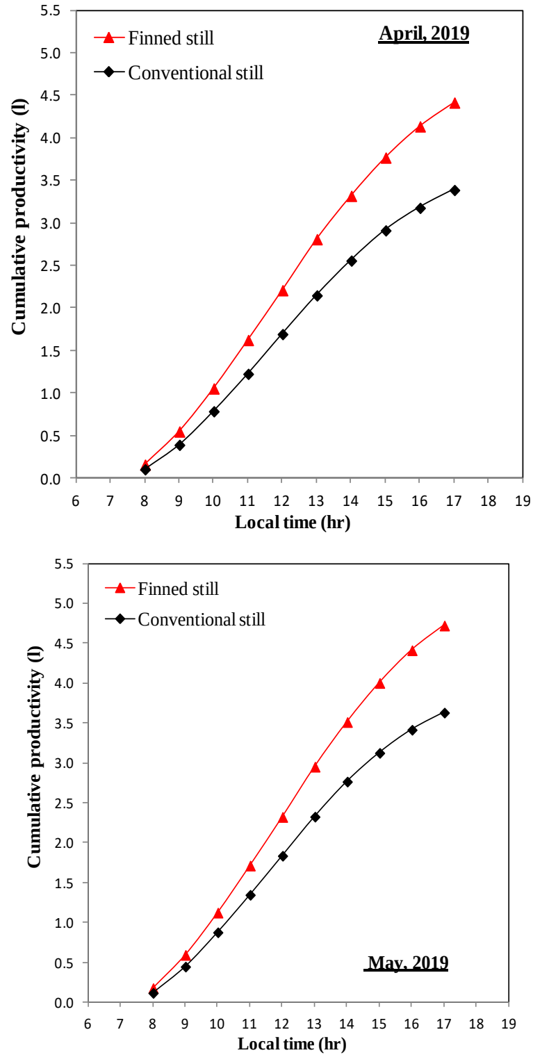
Figure 15. Variation of cumulative productivity from conventional and finned solar stills for February, March, April and May
