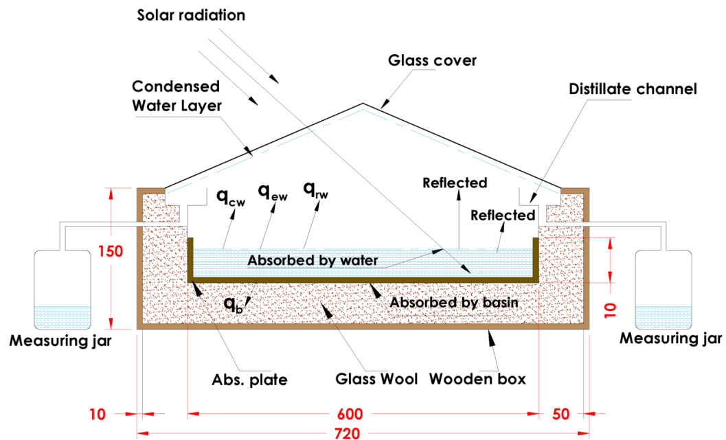
Figure 2. Schematic of the conventional solar still.
