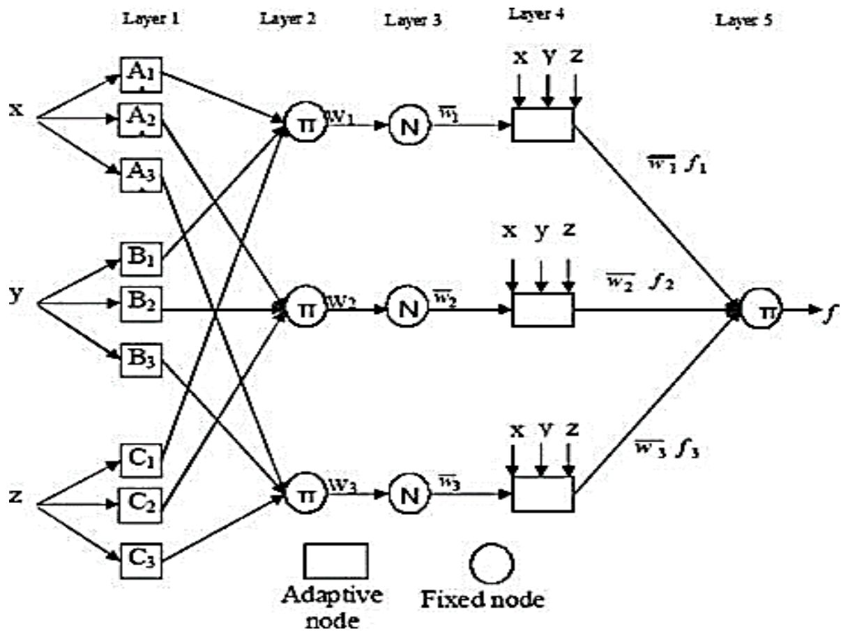
Figure 9. ANFIS structure.
