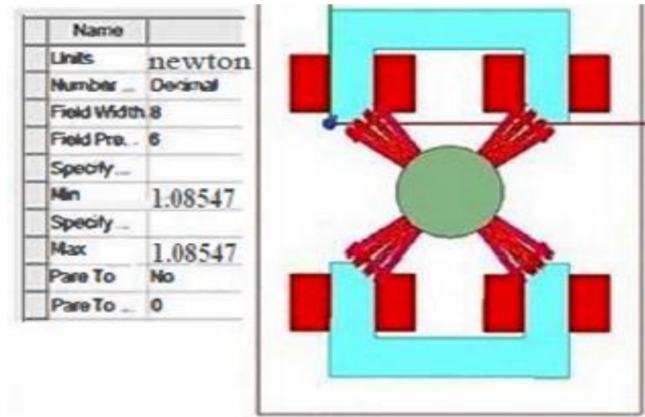
Figure 12. Force of the double-axis double coil U-type actuator.
