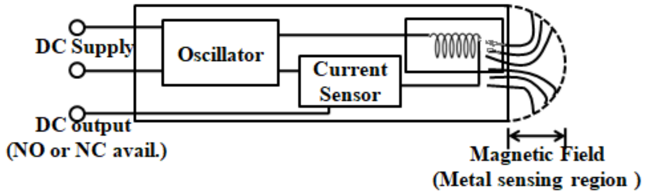
Figure 19. Schematic diagram of the inductive sensor.
