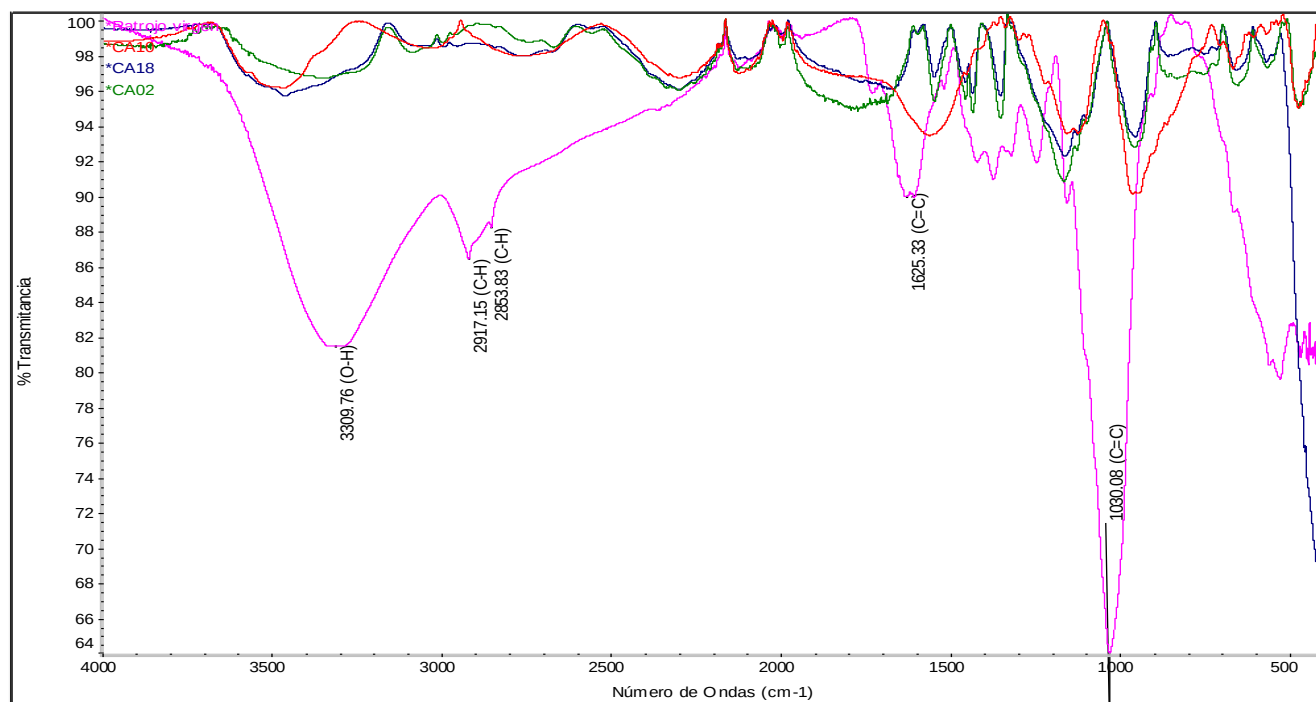
Figure 6. FTIR spectrum of treatment 2 corresponding to the use of \text{H}_3\text{PO}_4 , a ratio of 2:1 and without drying.
