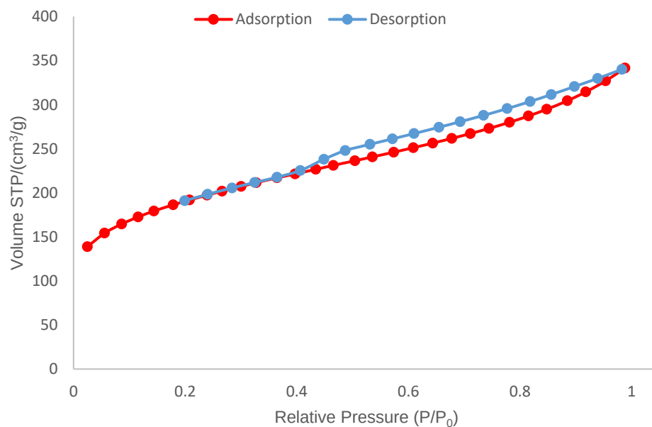
Figure 8. Nitrogen adsorption isotherm for the activated carbon sample produced with treatment 3 using \text{ZnCl}_2 as activating agent at a ratio of 4:1.
