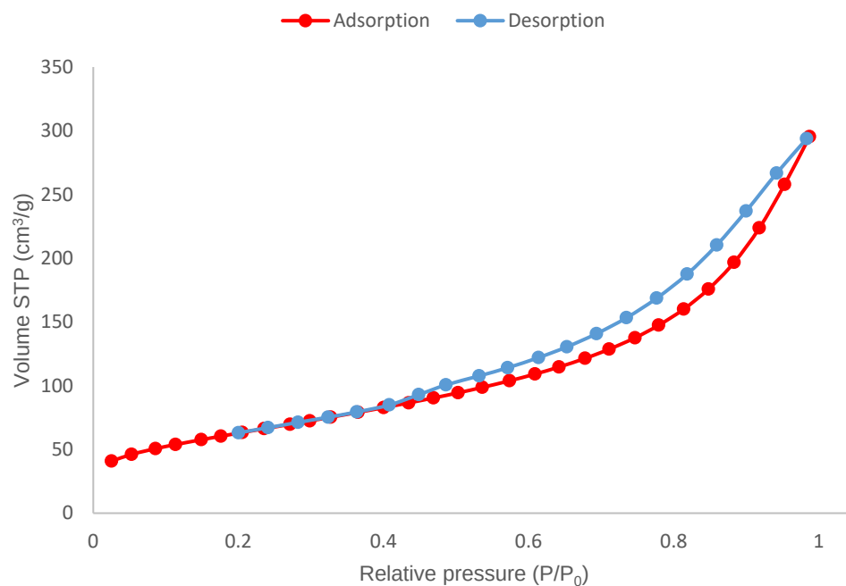
Figure 7. Nitrogen adsorption isotherm for the activated carbon sample produced with treatment 4 using \text{H}_3\text{PO}_4 as activating agent, at a ratio of 4:1.
