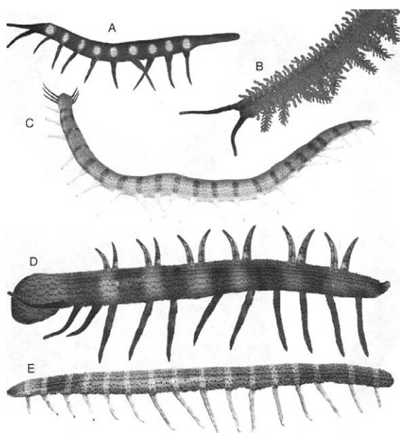
Fig. 4. Digital reconstructions of fossil onychophorans (Monge-Nájera & Xianguang, 2002). A: Microdictyon sinicum , B: Onychodictyon ferox , C: Cardiodictyon catenulum , D: Hallucigenia fortis , E: Luoishania lingicruris . Not to scale.
