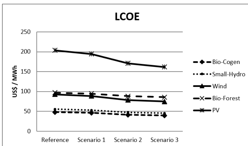
Figure 1 LCOE for three scenarios of incentives
