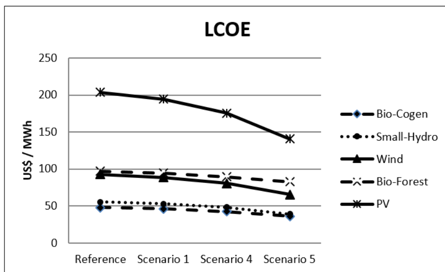
Figure 2 LCOE for additional scenarios of incentives Source: Authors' own creation
