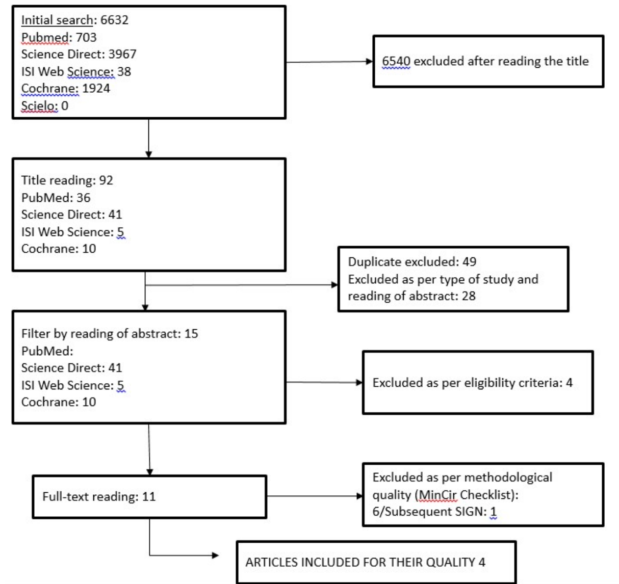
Figure 1: Search flowchart.
