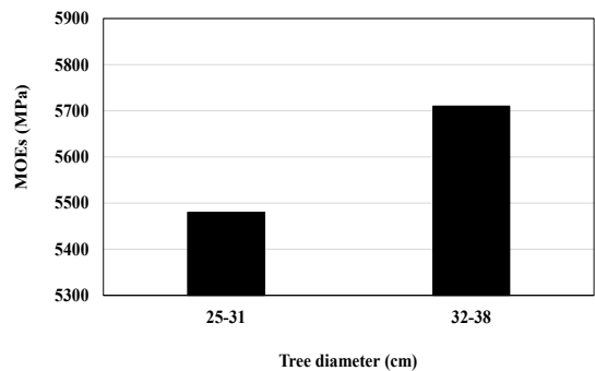
Figure 7: Effect of tree diameter on the static modulus of elasticity.
