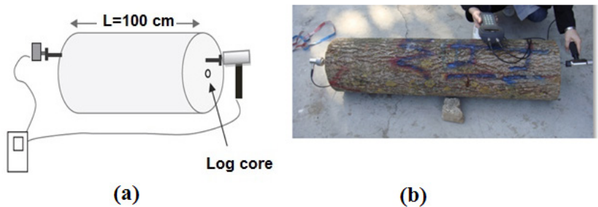
Figure 2: (a) Schematic and (b) real photo of log measurement using stress wave NDT.
