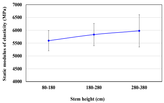
Figure 6: Modulus of elasticity in sawn wood of Paulownia.
