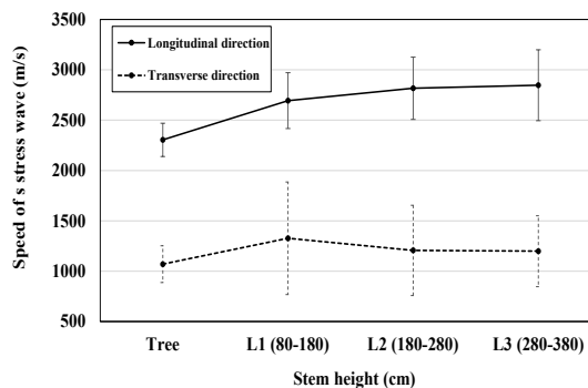
Figure 3: Stress wave velocity in trees and logs of Paulownia wood.
