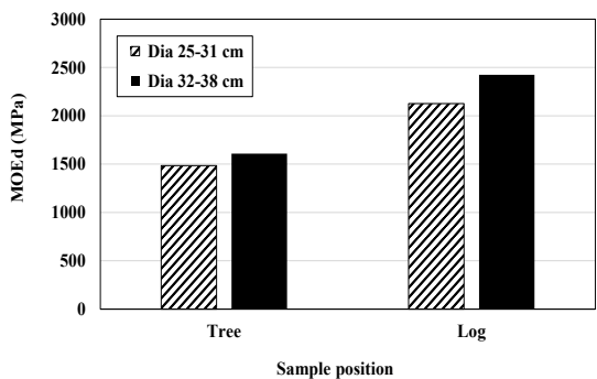
Figure 5: Effect of tree and log diameter on dynamic modulus of elasticity.
