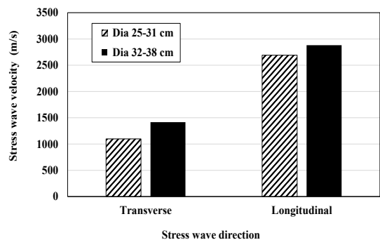
Figure 4: Effect of log diameter on stress wave velocity.
