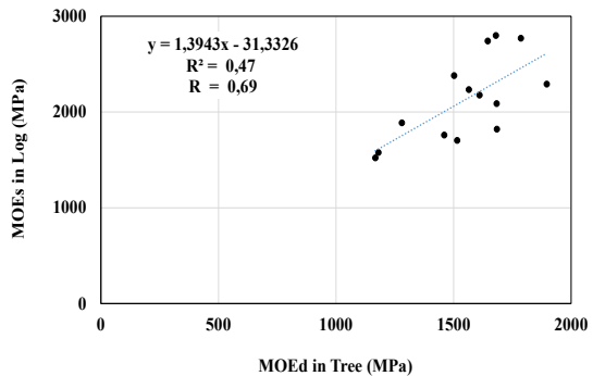
Figure 8: Relationship between MOE d in tree and log (L1) in Paulownia.
