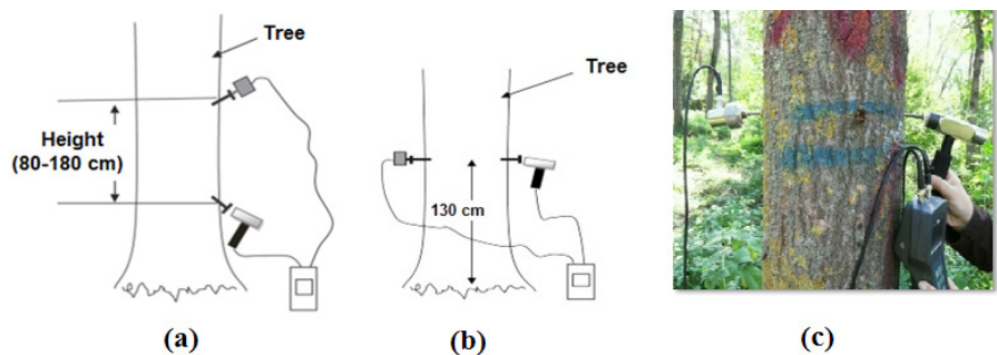
Figure 1: Schematic of tree measurement using stress wave NDT (a) longitudinal direction, (b) transverse direction and (c) real photo.
