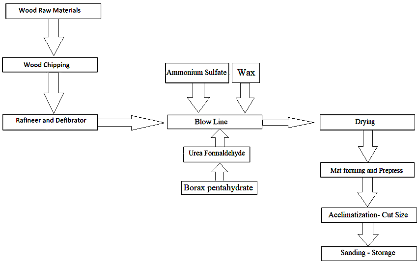
Figure 1: Product process flow sheet.
