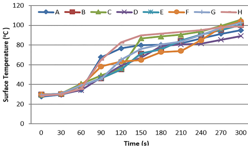
Figure 2: Surface temperature values of combustion experiment.
