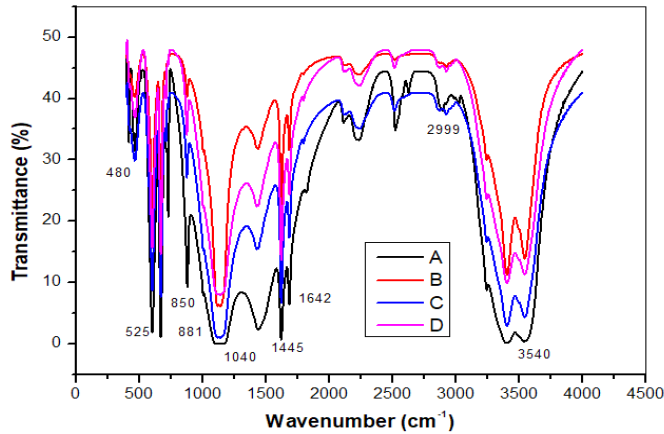
Figure 7: FTIR spectrum of board types A, B, C and D.
