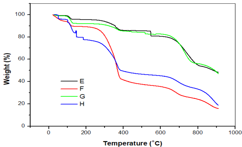
Figure 5: Thermogravimetric (TG) curves of board types E, F, G, H.
