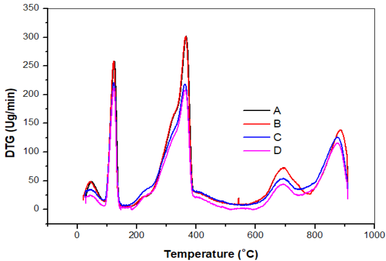
Figure 4: Derivative thermogravimetry (DTG) curves of board types A, B, C, D.
