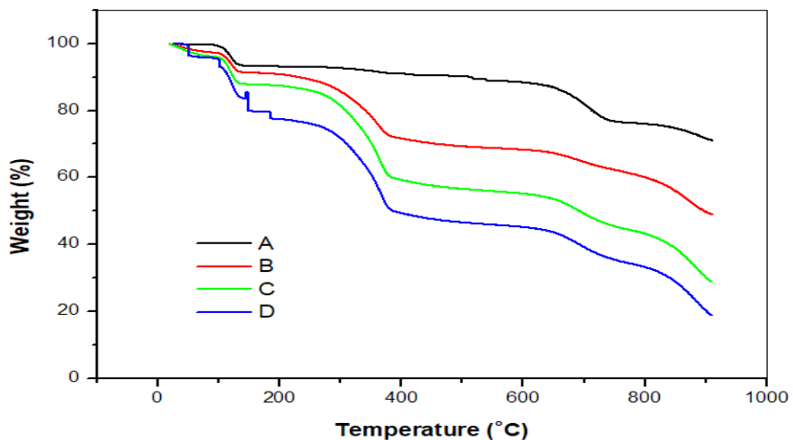
Figure 3: Thermogravimetric (TG) curves of board types A, B, C, D.
