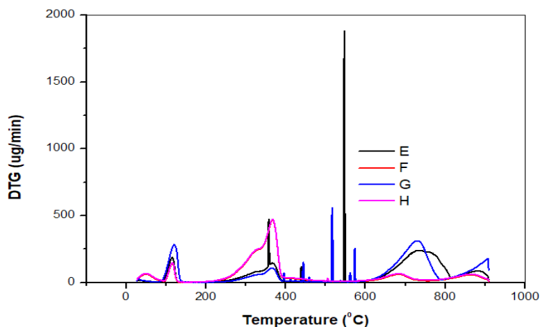
Figure 6: Thermogravimetry (DTG) curves of board types E, F, G, H.
