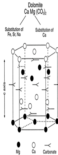
Figure 1: Calcium and magnesium ions in the structure of dolomite (Warren 2000).
