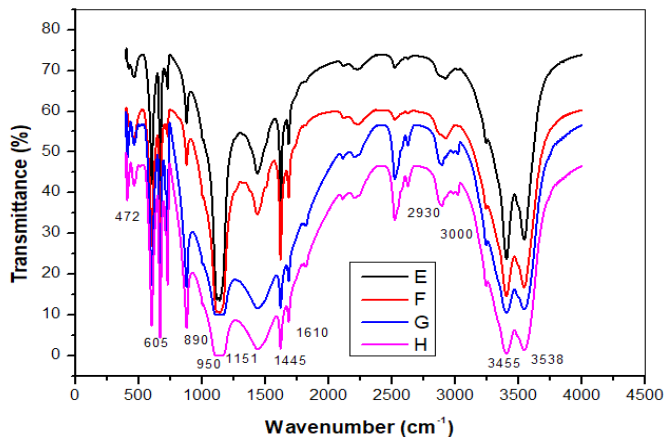
Figure 8: FTIR spectrum of board types E, F, G and H.
