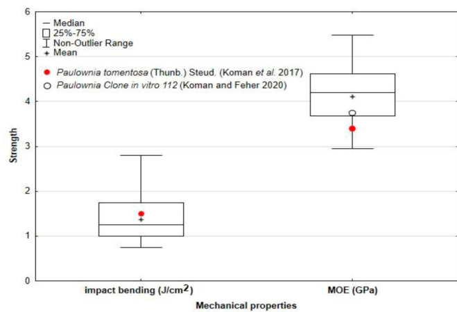
Figure 3: Impact bending strength and modulus of elasticity of the examined paulownias.
