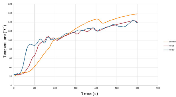
Figure 3: Inner layer temperature chart of the treatments performed.
