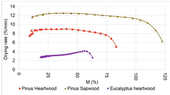
Figure 7: Effect of moisture content on drying rate.
