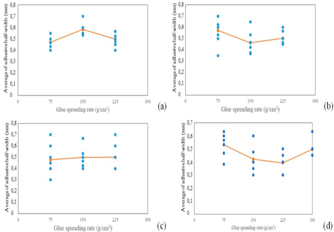
Figure 7: PF adhesive half-width of (a) low density heartwood plywood, (b) medium density heartwood plywood, (c) high density heartwood plywood, and (d) medium density sapwood plywood.
