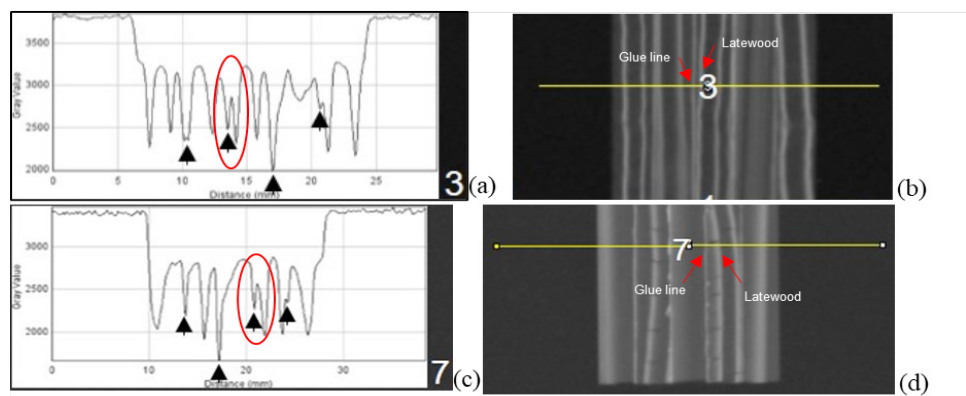
Figure 8: The X-ray image and its plot profile which indicates the smallest half-width value (0,3 mm). (a) A plot profile of medium veneer density of sapwood plywood with 150 g/m 2 glue spreading rate and (b) its X-ray image, and (c) a plot profile of high veneer density of heartwood plywood with 75 g/m 2 glue spreading rate and (d) its X-ray image.
