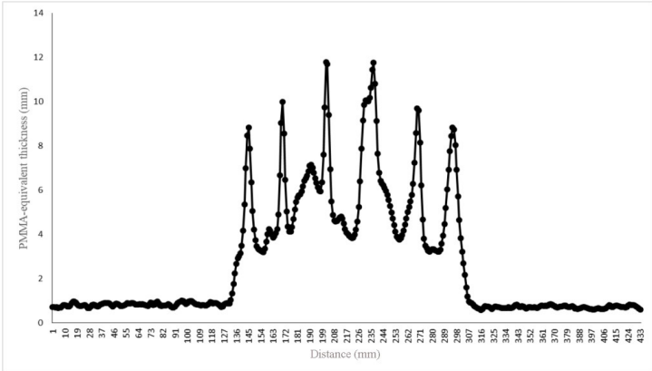
Figure 4: The plot profile of line 6 in high density heartwood plywood with 225 g/cm 2 glue spreading rate that successfully converted using PMMA equation from PMMA calibration curved. After converting the plot profile, the mechanism for calculating the penetration depth of the glue was developed in this study and is shown in Figure 5.
