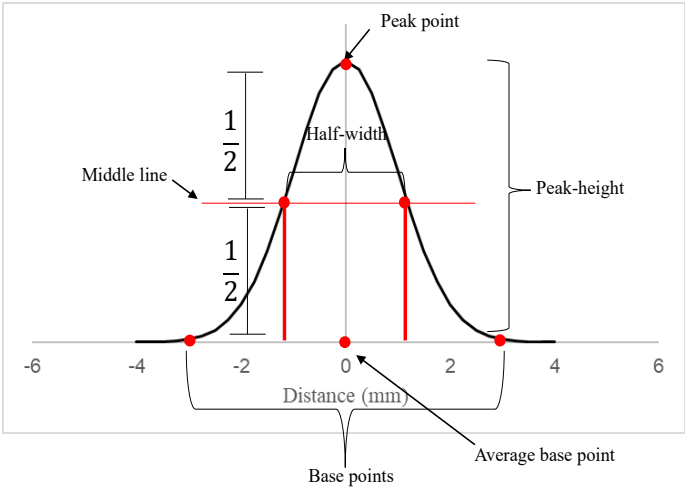
Figure 5: The mechanism of calculated the peak height and half-width. The base point of the peak should be determined based on the horizontal inequality position of the base point. After the peak height was obtained, the height of the graph was divided by two, which was the way to obtain the middle line of the graph. Then, the length of the middle line of the graph, which is defined as the half-width occurred. The half-width of the peak was considered as the adhesive penetration depth. The peak height was considered as the adhesive concentration. The half-width and peak-height were obtained from the calculation of the glue line peak (Figure 6). The half-width (adhesive penetration) value obtained from various glue spreading rate and veneer density was investigated to see the relations between them (Figure 7).
