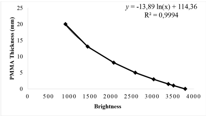
Figure 2: Equation of the PMMA-equivalent thickness.
