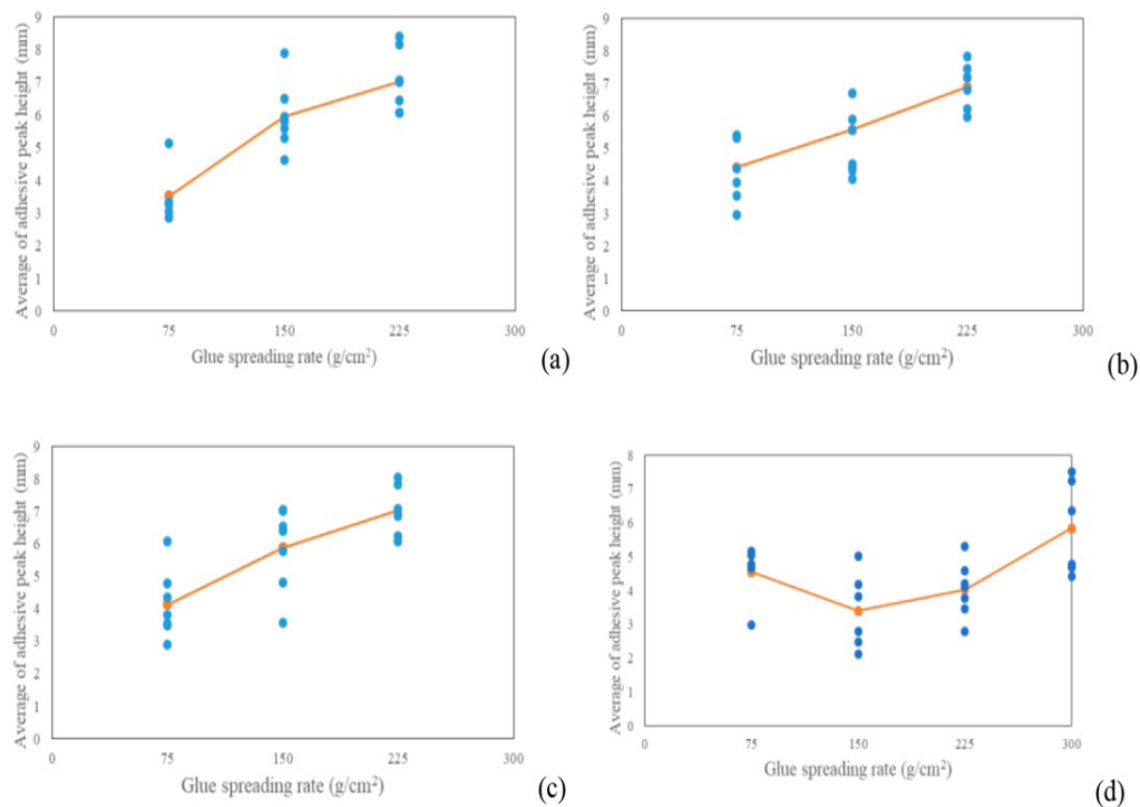
Figure 9: PF adhesive peak height of (a) low density heartwood plywood, (b) medium density heartwood plywood, (c) high density heartwood plywood, and (d) medium density sapwood plywood.
