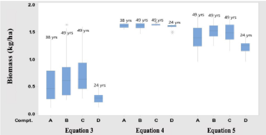
Figure 5: The relevance of variance between the Equation 3, Equation 4 and Equation 5.
