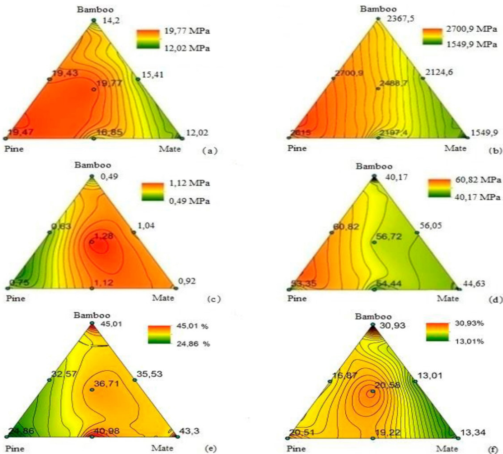
Figure 3: Modulus of rupture in static bending (a) Modulus of elasticity in static bending (b), Internal bond strength (c), Janka hardness (d), Water absorption (e) and Thickness swelling (f) of High-Density Particleboard (HDP).
