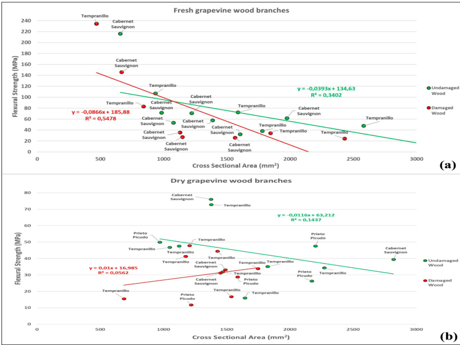
Figure 4: Linear regression of the flexural strength (FS) (MPa, y-axis) (A, fresh; B, dry) in relation to cross sectional area (CSA) (mm², x-axis) in grapevine branches. 'Green Points' represent values for grapevine branch samples of different varieties undamaged by X. arvicola larvae; 'Red Points' represent values for grapevine branch samples of different varieties damaged by X. arvicola larvae. 'Green Line' is the trendline for 'Green Points'; 'Red Line', is the trendline for 'Red Points'.
