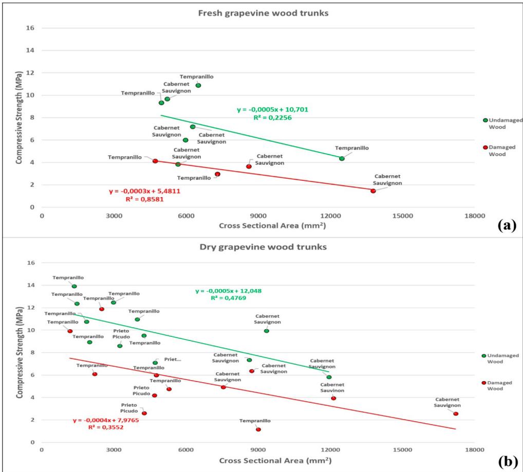
Figure 3: Linear regression of the compressive strength (CS) (MPa, y-axis) (a) fresh; (b) dry) in relation to cross sectional area (CSA) (mm², x-axis) in grapevine trunks. ‘Green Points’ represent values for trunk samples of different varieties undamaged by X. arvicola larvae; ‘Red Points’ represent values for trunk samples of different varieties damaged by X. arvicola larvae. ‘Green Line’ is the trendline for ‘Green Points’; ‘Red Line’ is the trendline for ‘Red Points’.
