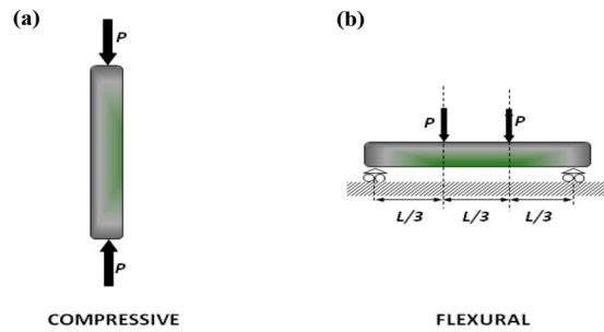
Figure 1: (a) Load diagram for compressive tests in grapevine trunks ( P uniaxial forces were applied by a constant load speed of 200 N/s up to failure); (b) Load diagrams for flexural tests in grapevine branches (the two P forces were applied in the central third of the sample by a constant load speed of 200 N/s up to failure. 'i', and 'ii' were the roller supports of the wood samples).
