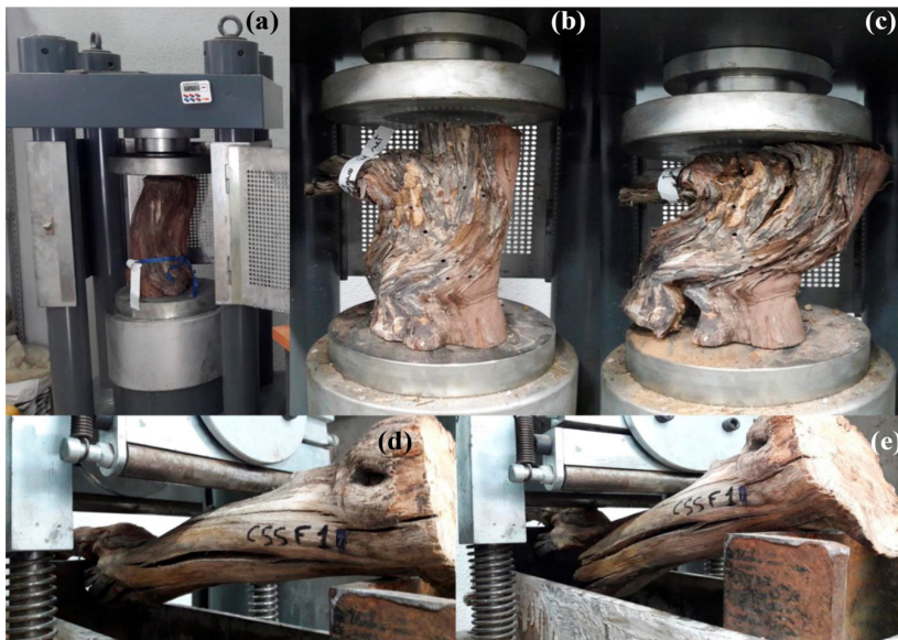
Figure 2: (a) Pictorial illustration of the hydraulic press used for compressive and flexural tests; (b) affected grapevine trunk before compressive test; (c) affected grapevine trunk after compressive test; (d) affected grapevine branch before flexural test; (e) affected grapevine branch after flexural test.
