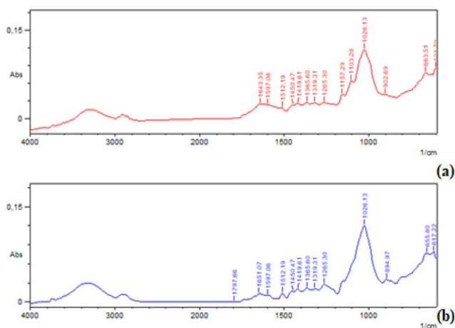
Figure 4: ATR-FTIR spectra for molding- Pinus sylvestris : (a) outer surface, (b) inner surface.
