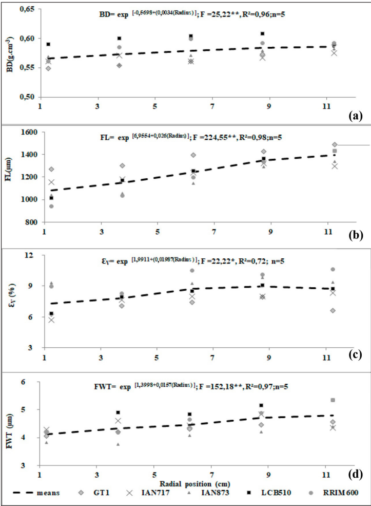
Figure 2: Correlation between (a) basic density and radial position; (b) fiber length and radial position, (c) volumetric shrinkage and radial position, and (d) fiber wall thickness and radial position of 33-year-old Hevea brasiliensis .
